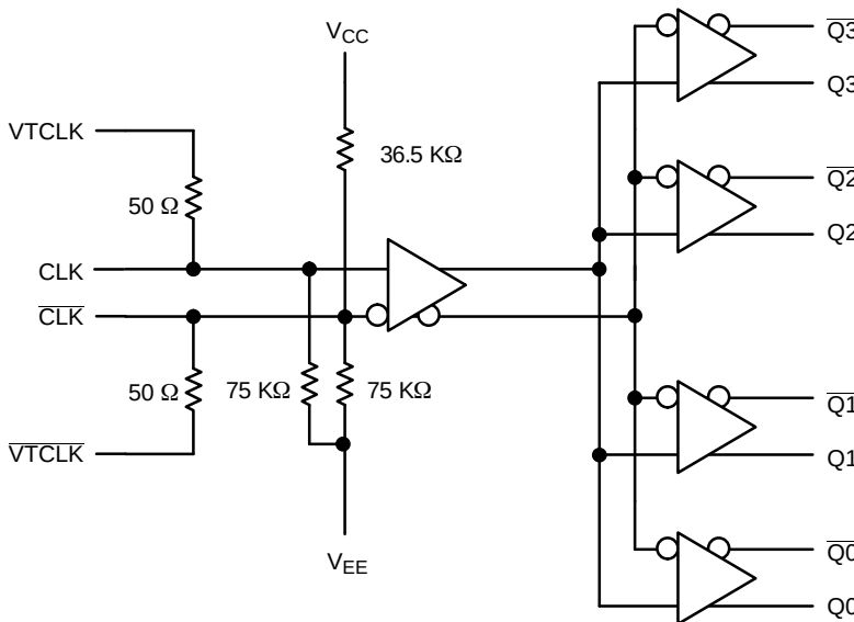
Figure 2. Logic Diagram
