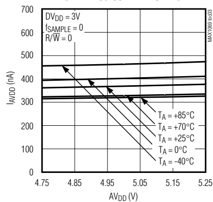
ANALOG SHUTDOWN CURRENT vs. ANALOG SUPPLY VOLTAGE
