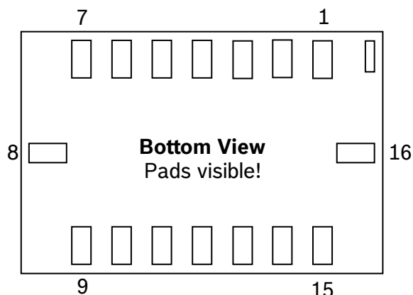
Figure 30: Pin-out bottom view
