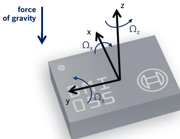
Figure 35: Orientation of sensing axis
