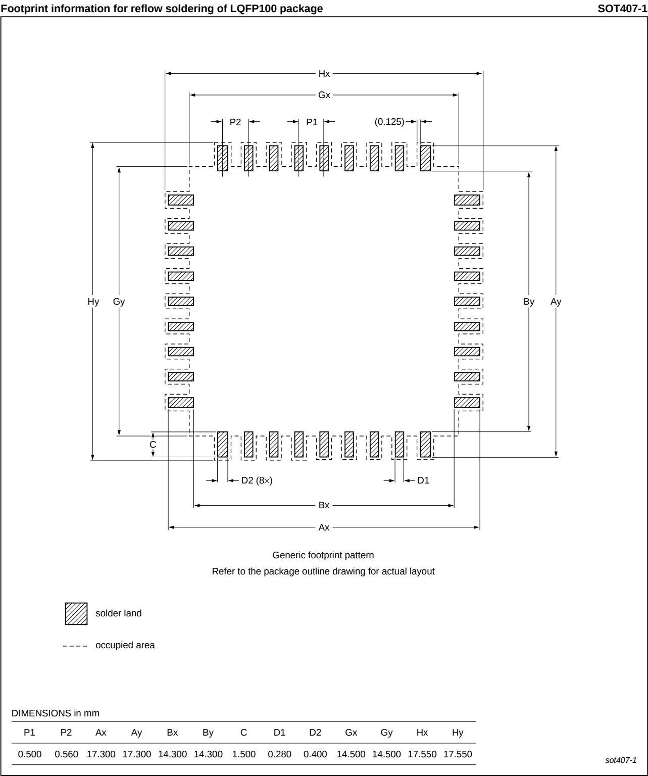
Fig 55. Reflow soldering of the LQFP100 package
