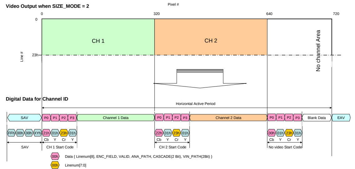
Fig 47 The digital channel ID format in channel boundary
