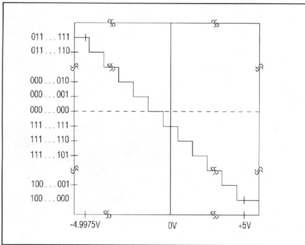
Figure 21. Inverting Bipolar Transfer Function
