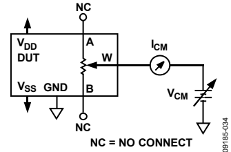
Figure 33. Common-Mode Leakage Current
