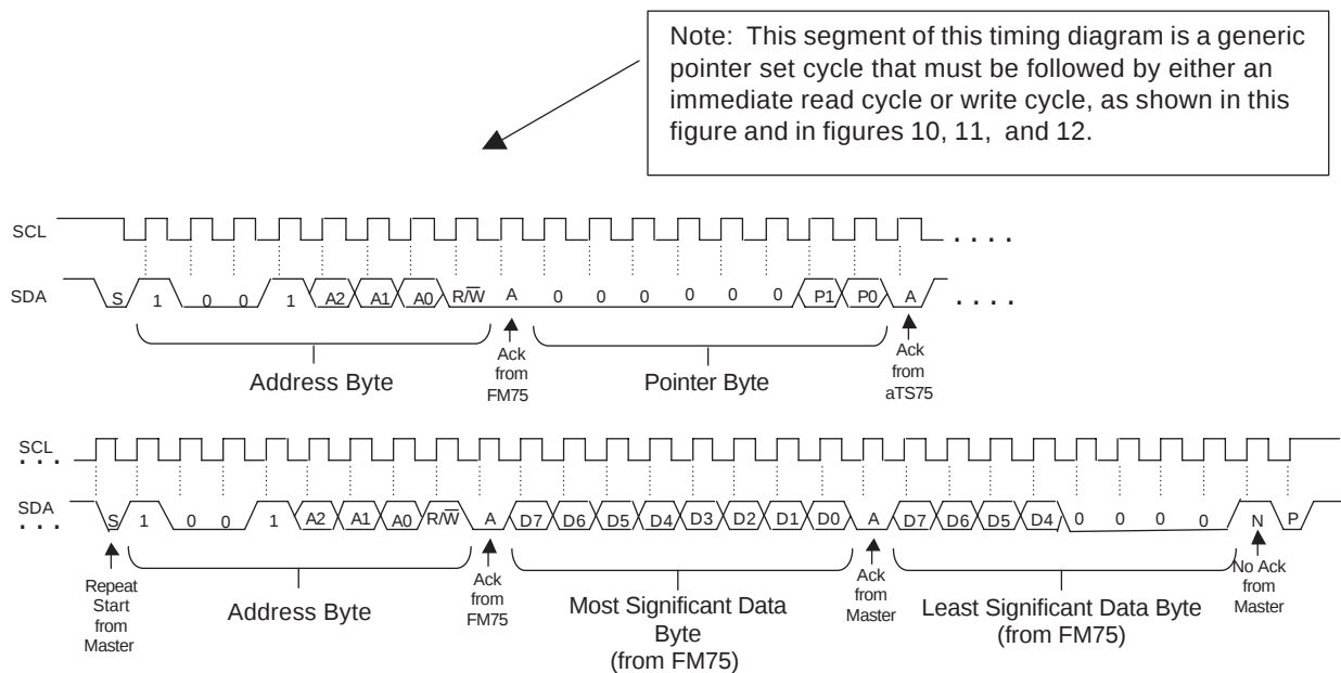
Figure 11. Pointer Set Followed by Immediate Read from a Two-byte Register (Temperature, T_{OS} , or T_{HYST} Register)
