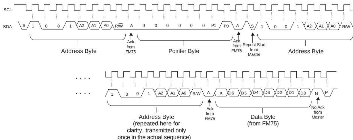
Figure 15. Pointer Set Followed by Immediate Read from Configuration Register
