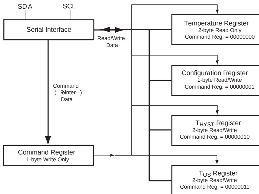
Figure 5. Register Hierarchy
