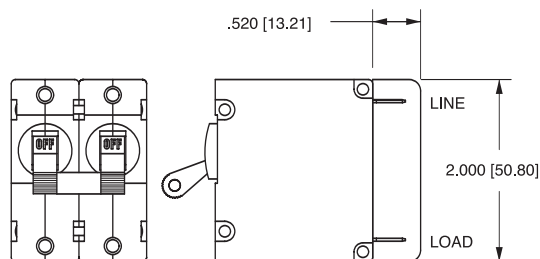
BARRIER FOR UL-RECOGNIZED MULTI-POLE BREAKERS
