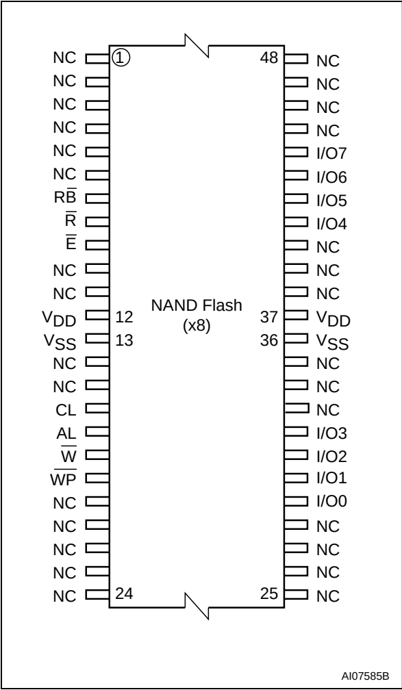
Figure 4. TSOP48 and WSOP48 Connections, x8 devices
