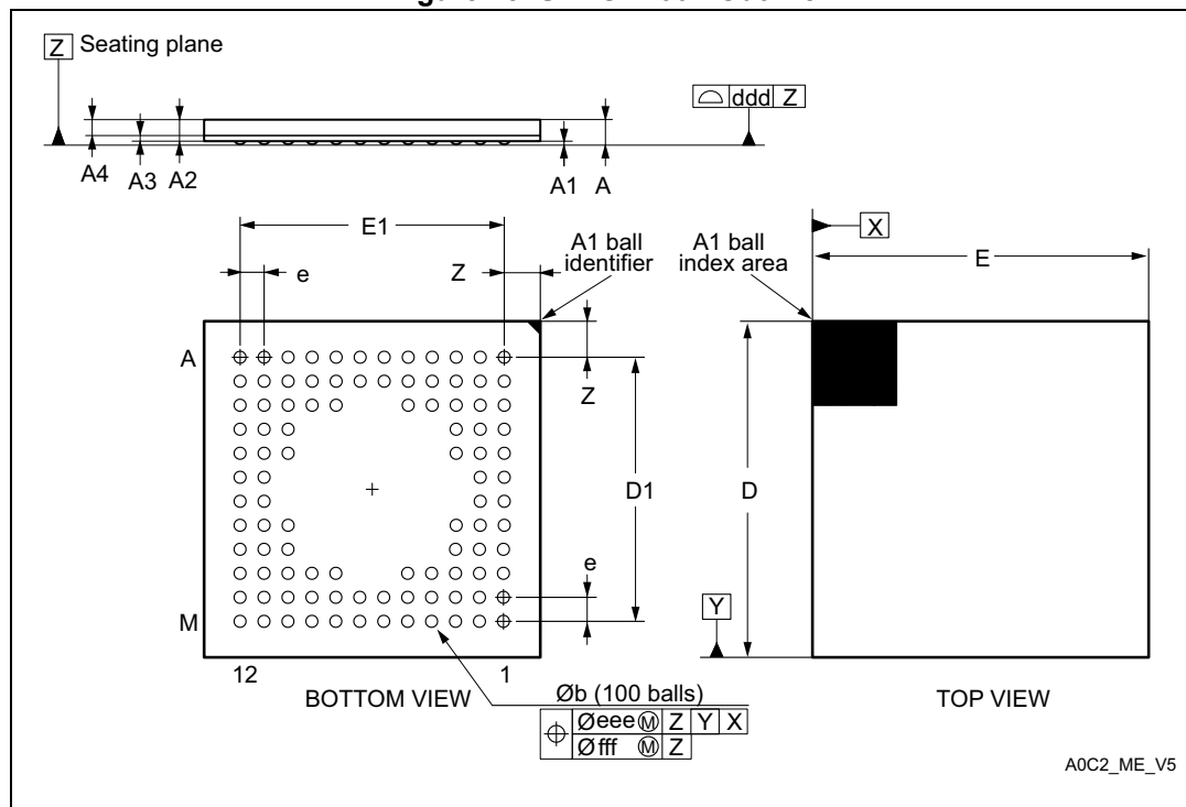
Figure 43. UFBGA100 - Outline
