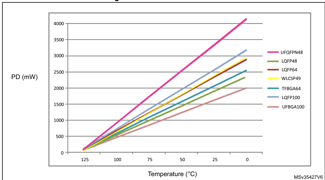
Figure 61. Thermal resistance
