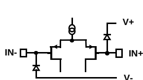
CIRCUIT 1
