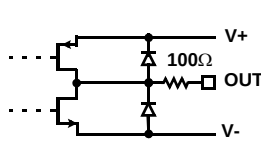
CIRCUIT 3
