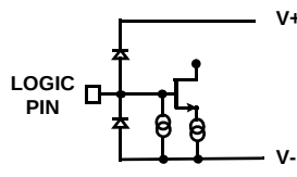
CIRCUIT 2
