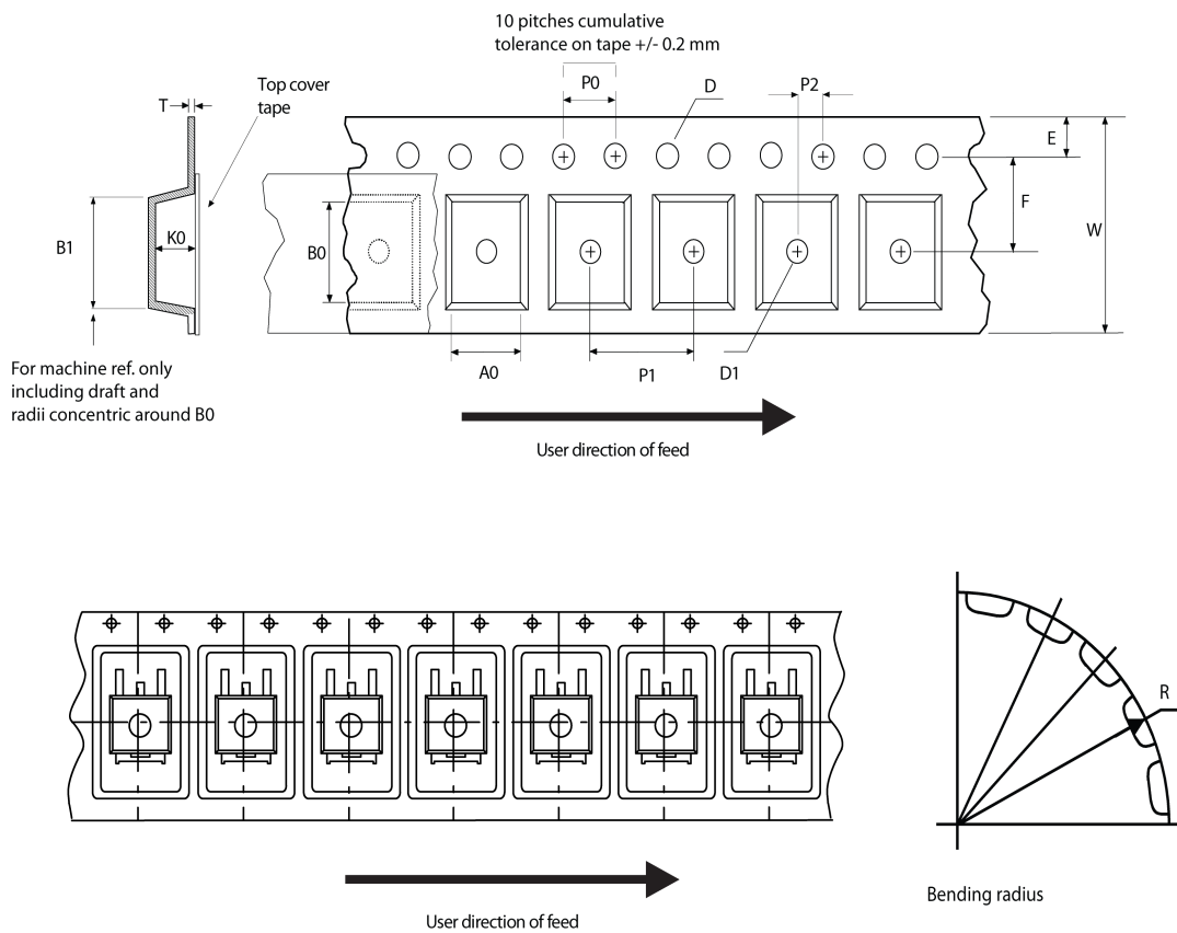
Figure 47. Tape outline
