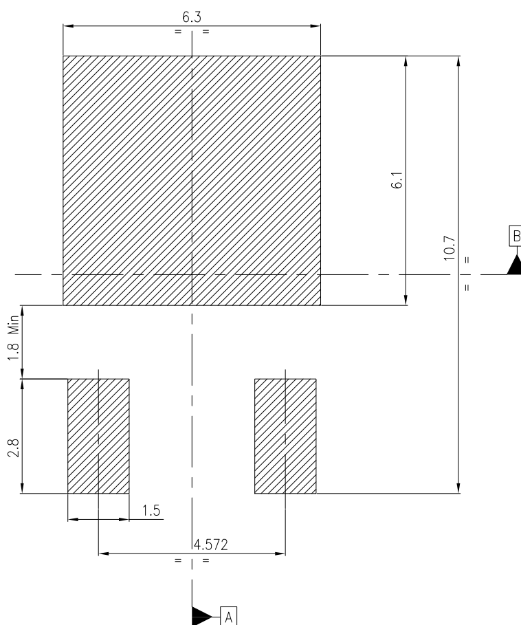
Figure 43. DPAK recommended footprint (dimensions are in mm)
