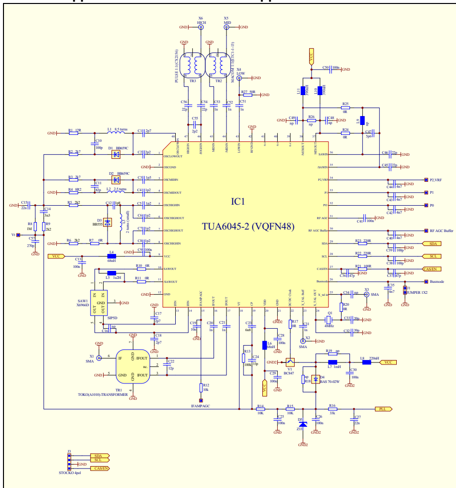
Figure 6 Circuit diagram for L-Band application
