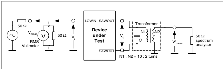
Figure 9 Gain ( G_V ) measurement in LOW band
