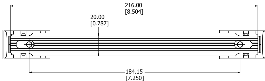
BOTTOM VIEW
