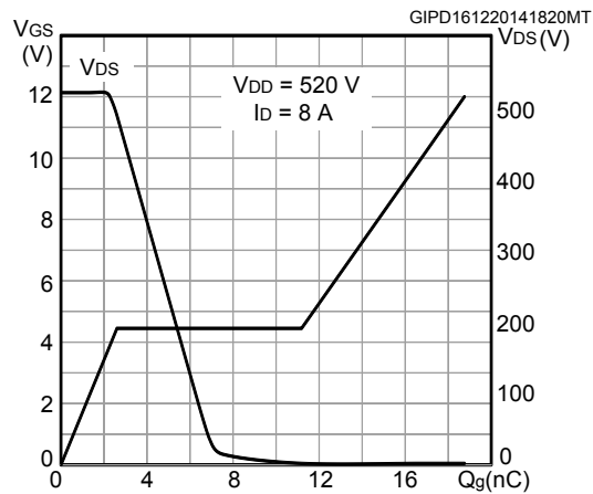
Figure 9. Typical gate charge characteristics
