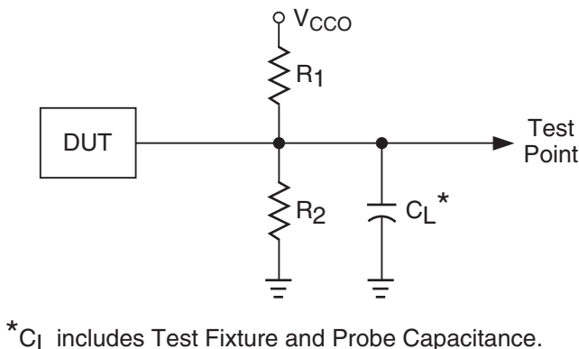
Figure 9. Output Test Load, LVTTTL and LVCMOS Standards
