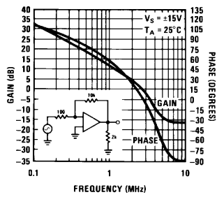
Bode Plot LM149
