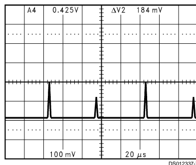
FIGURE 3. Measurement of the Shoot-Through Current
