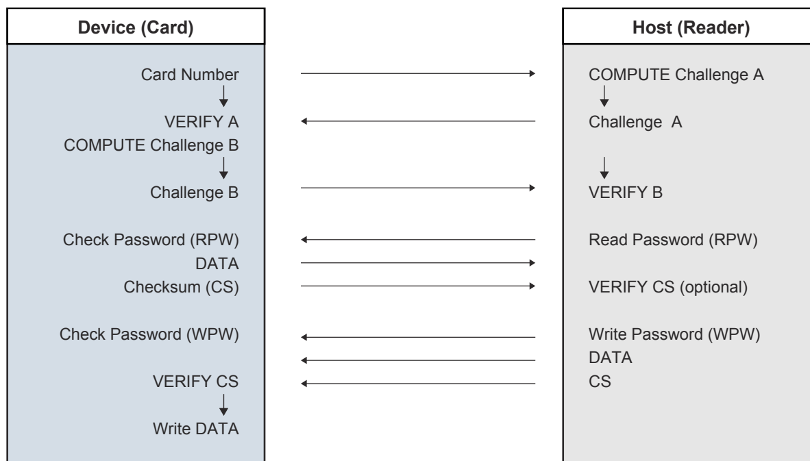
Figure 3. Security Methodology
