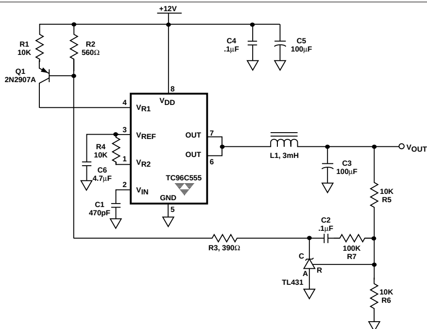
Figure 5. +5V Buck Regulator Power Supply with 82% Efficiency at 200mA Output
