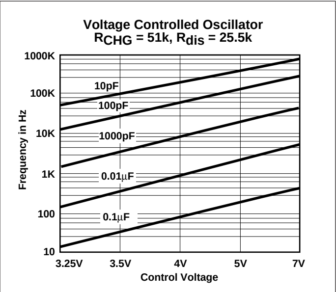
Figure 8. Frequency vs Control
