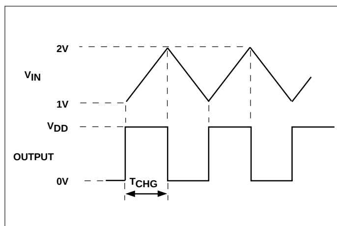
Figure 3. V_{IN} and Output Waveform
