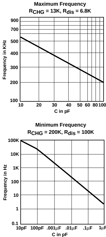
Figure 4. Typical Maximum and Minimum Operating Frequency vs. Capacitor
