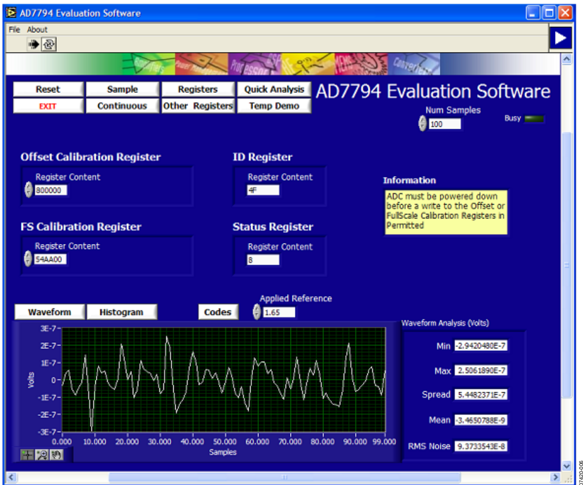
Figure 5. AD7794 Evaluation Software Other Registers Window
