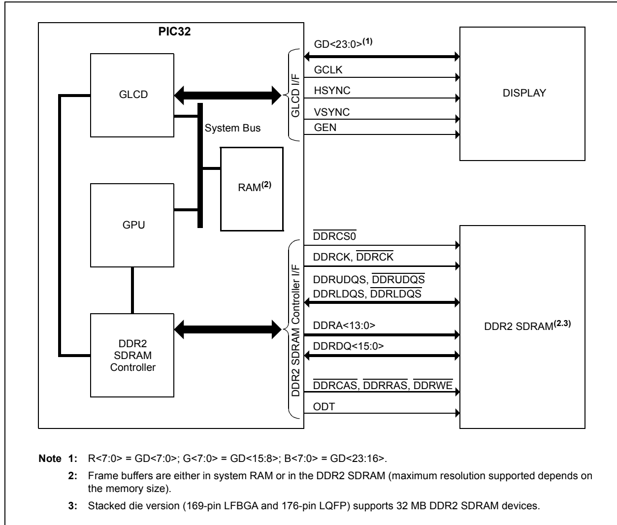
FIGURE 2-6: GRAPHICS APPLICATION
