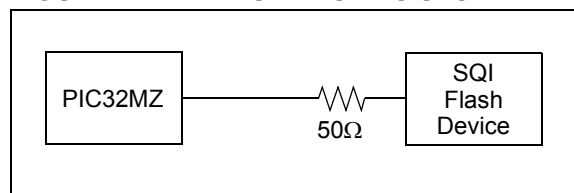
FIGURE 2-4: SERIES RESISTOR
