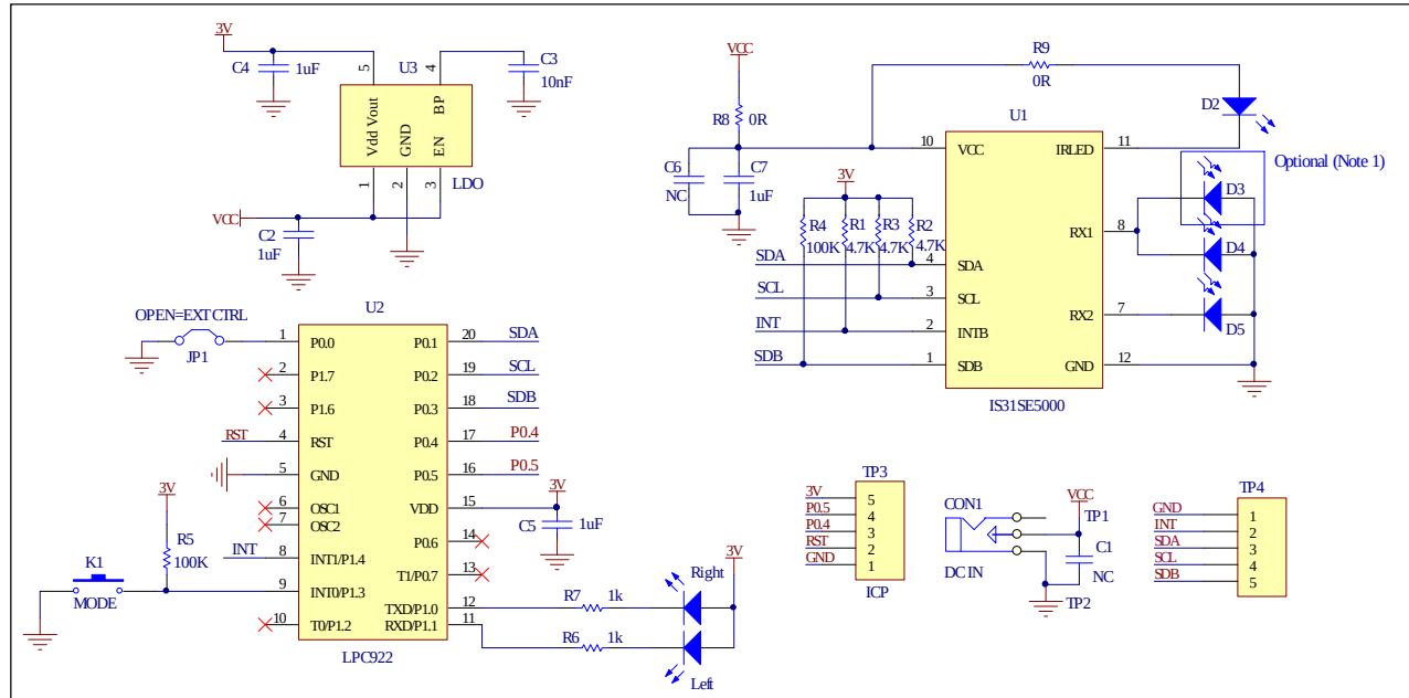
Figure 2: IS31SE5000 Application Schematic
