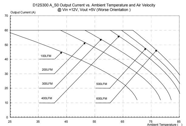
Figure 39: Output current vs. ambient temperature and air velocity @ Vin=12V, Vout=5V (Worse Orientation)
