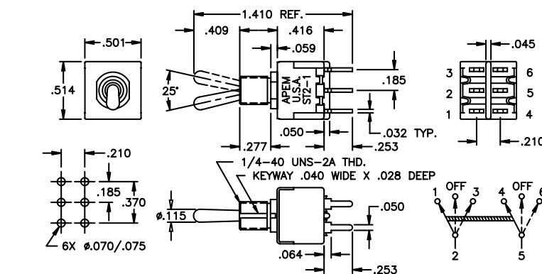
DOUBLE POLE
