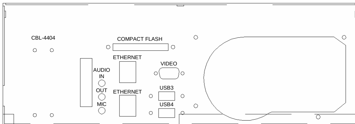
Figure 5. VL-ENCL-5 Back Panel (All Models)
