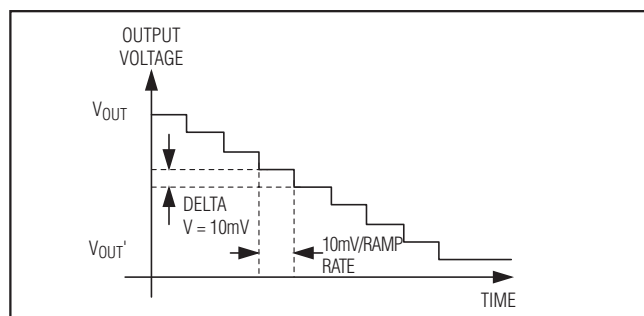
Figure 7. Ramp-Down Function
