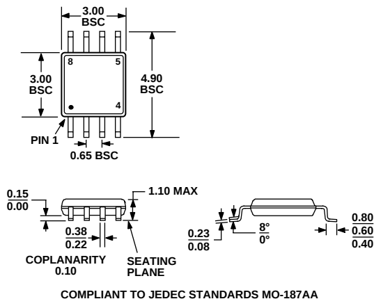
Figure 59. 8-Lead Mini Small Outline Package [MSOP] (RM-8)
