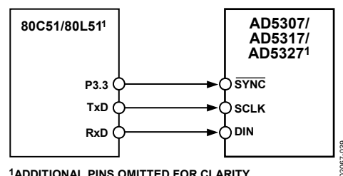
Figure 39. 80C51/80L51-to-AD5307/AD5317/AD5327 Interface
