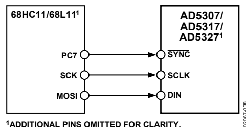
Figure 38. 68HC11/68L11-to-AD5307/AD5317/AD5327 Interface
