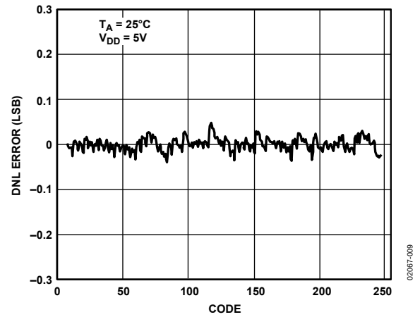
Figure 9. AD5307 DNL
