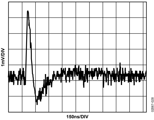
Figure 28. DAC-to-DAC Crosstalk
