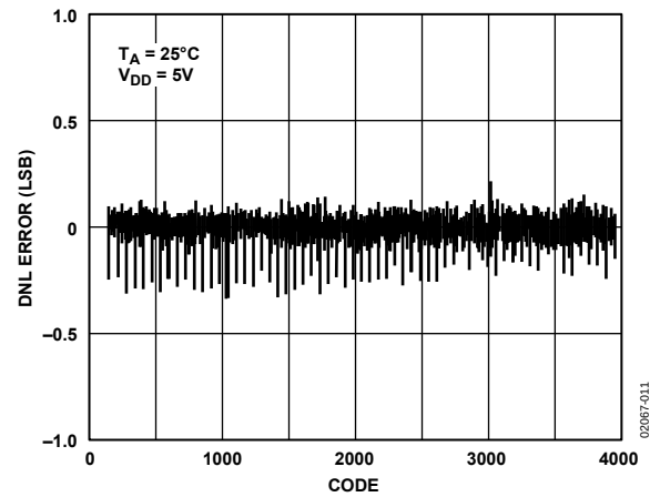
Figure 11. AD5327 DNL
