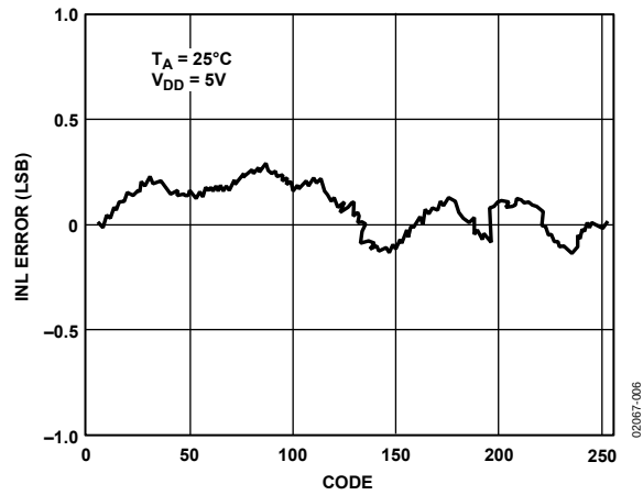
Figure 6. AD5307 INL
