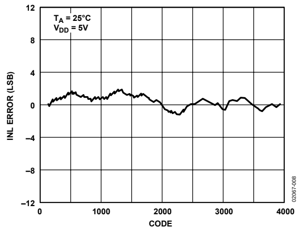
Figure 8. AD5327 INL
