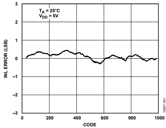
Figure 7. AD5317 INL
