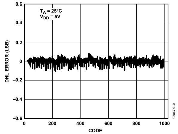
Figure 10. AD5317 DNL
