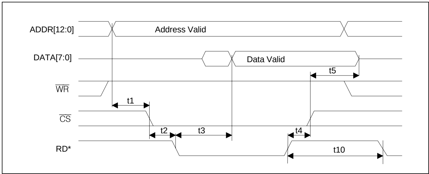
Figure 19-7 Intel Bus Read Timing (BTS = 0)
