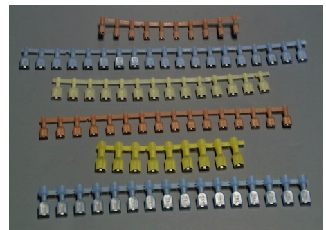
Quixon Fully-Insulated Quick-Disconnect Terminals (Red = 18 to 22 AWG; Blue = 14 to 16 AWG; Yellow = 10 to 12 AWG)
