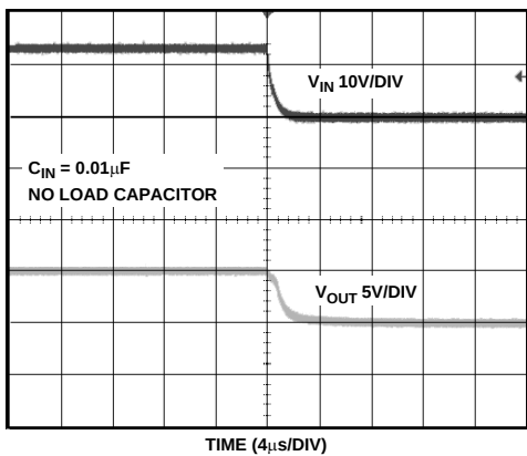
Figure 30. ADR02 Turn-Off Response
