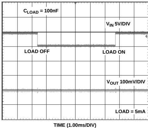
Figure 29. ADR02 Load Transient Response
