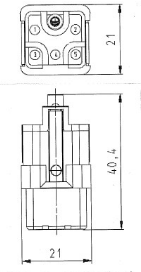
26.06.2013 Drawing Dimensions in mm (Inch)
