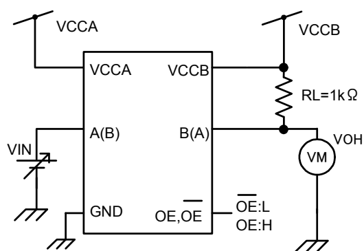
Figure 7 Test Circuit
