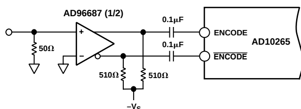
Figure 20. ECL Comparator for Encode
