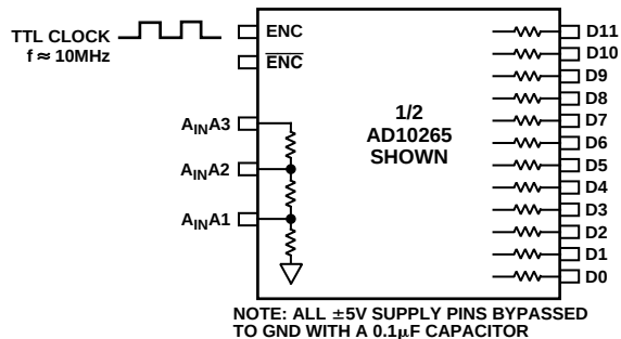
Figure 2. Equivalent Burn-In Circuit
