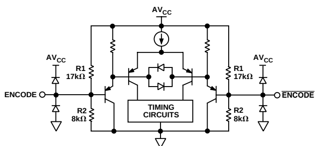
Figure 4. Encode Inputs
