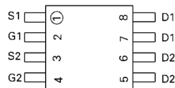
Top View Pin-Out
