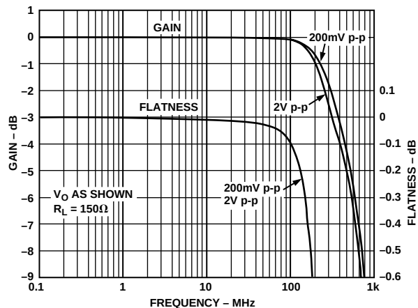
Figure 3. AD8183 Frequency Response; R_L = 150 \Omega
