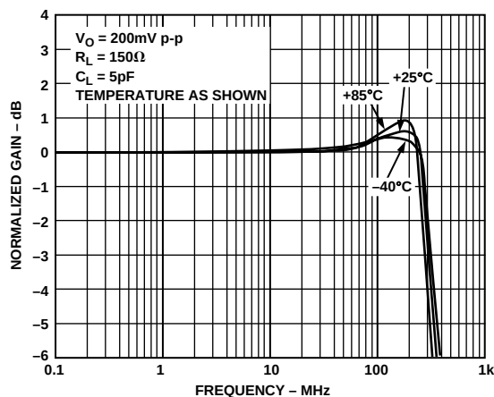
Figure 8. AD8185 Frequency Response vs. Temperature
