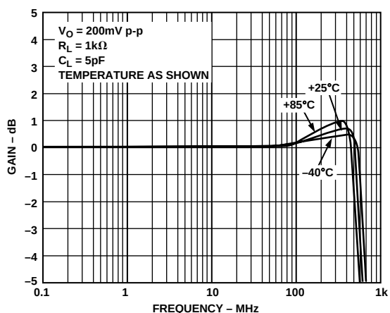
Figure 5. AD8183 Frequency Response vs. Temperature
