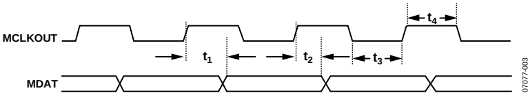
Figure 3. Data Timing
