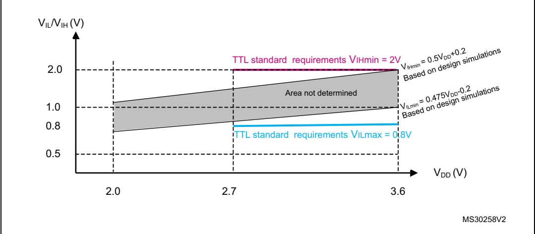
Figure 22. Five volt tolerant (FT and FTf) I/O input characteristics - TTL port
