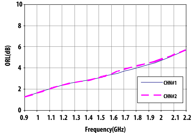
Figure 10. ORL vs Frequency vs Channel
