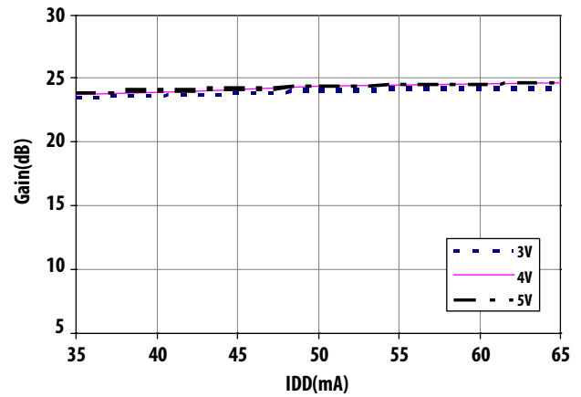
Figure 18. Gain vs IDD vs VDD
