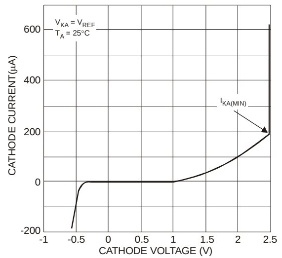
Cathode Current (μA) vs. Cathode Voltage
