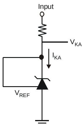
Figure. 1 Test Circuit for V_{KA} = V_{REF}
