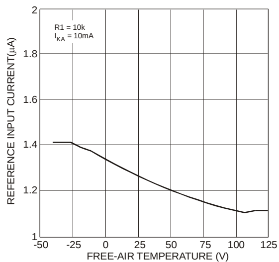
Reverence Input Current vs. Free Temperature
