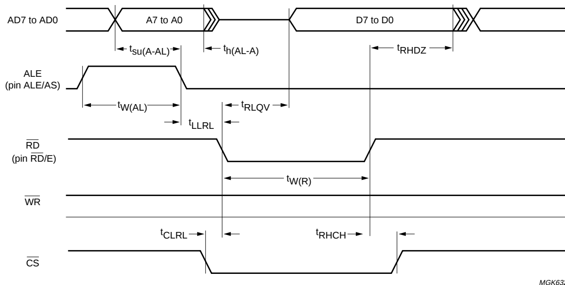
Fig.17 Read cycle timing diagram; Intel mode.
