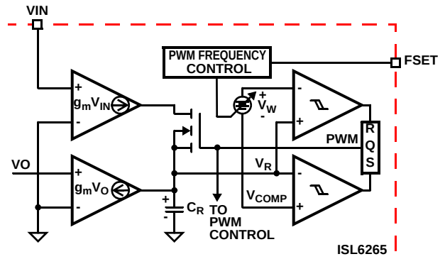
FIGURE 5. MODULATOR CIRCUITRY
