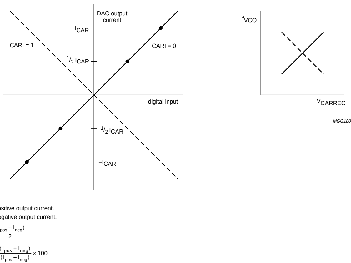
Fig.10 Definition of the DAC currents and the expected frequency behaviour of the VCO.
