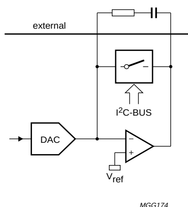
Fig.15 Loop amplifier and analog switch.
