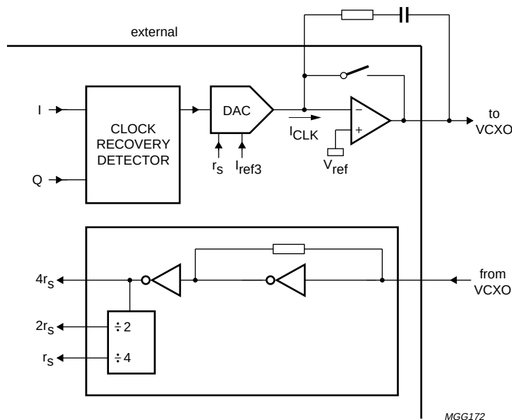
Fig.11 Schematic diagram of the clock recovery.
