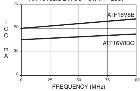
SUPPLY CURRENT vs. INPUT FREQUENCY ATF16V8B/BQ (VCC = 5V, TA = 25C)
