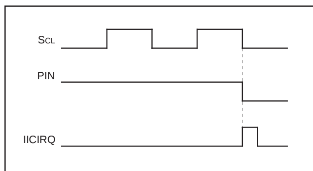
Fig. 24 Interrupt request signal generating timing
