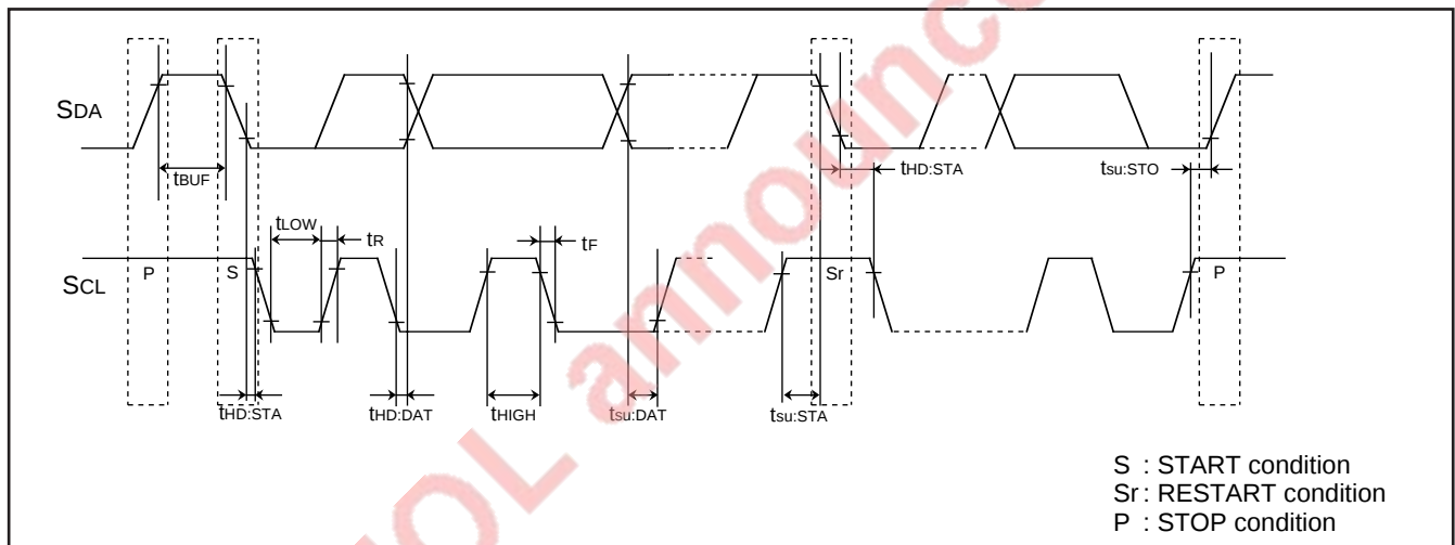
Fig. 52 Timing diagram of multi-master I 2 C-BUS
