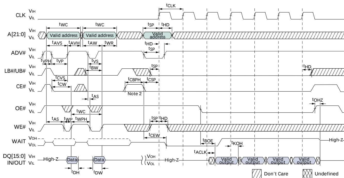
Figure 50: Asynchronous WRITE Followed by Burst READ
