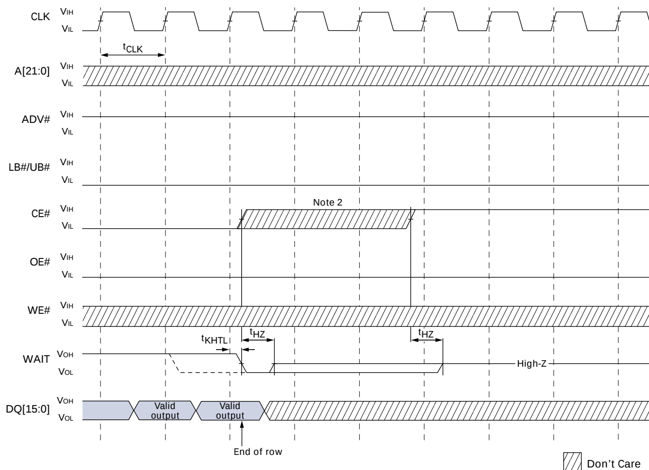
Figure 38: Burst READ at End-of-Row (Wrap Off)
