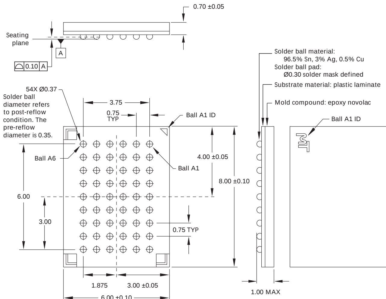
Figure 56: 54-Ball VFBGA
