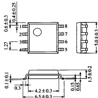
8-pin PANAFLAT Plastic Package (SO-8D) (SOP008-P-0255A)
