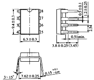
8-pin DIL Plastic Package (DIP008-P-0300B)
