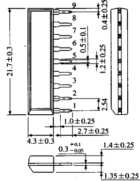
9-pin SIL Plastic Package (Slim) (SIP009-P-0000A)
