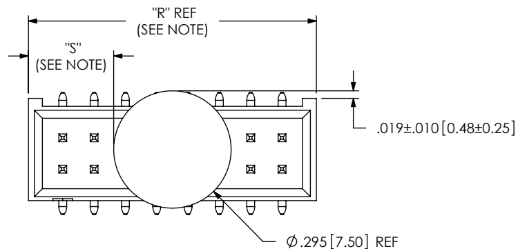
FIG 6 -K OPTION (POLYIMIDE FILM) LTMM-108-01-XX-D-SM-K SHOWN FOR SURFACE MOUNT OPTIONS ONLY (DIFFERENT AS SHOWN, OTHERWISE SAME AS FIG 3)
