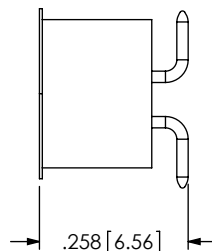
FIG 6 -K OPTION (POLYIMIDE FILM) LTMM-108-01-XX-D-SM-K SHOWN FOR SURFACE MOUNT OPTIONS ONLY (DIFFERENT AS SHOWN, OTHERWISE SAME AS FIG 3)
