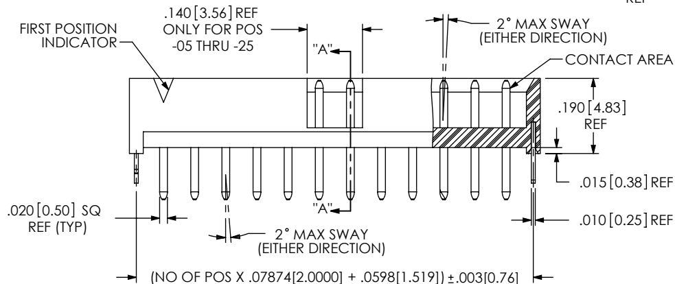
FIG 1 THROUGH HOLE LTMM-112-02-XX-D-LC SHOWN
